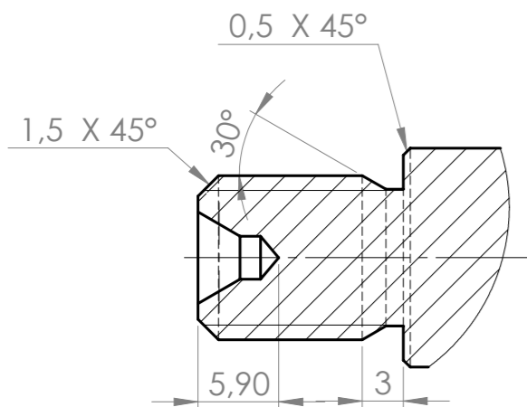
DETAIL B SCALE 2 : 1 Ens i begge ender
